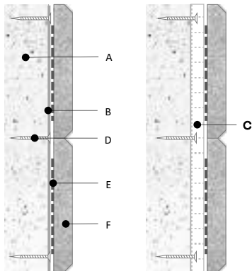
WM-A – Metal Sheets
