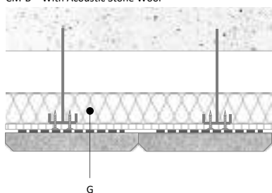
CM-B – With Acoustic Stone Wool
